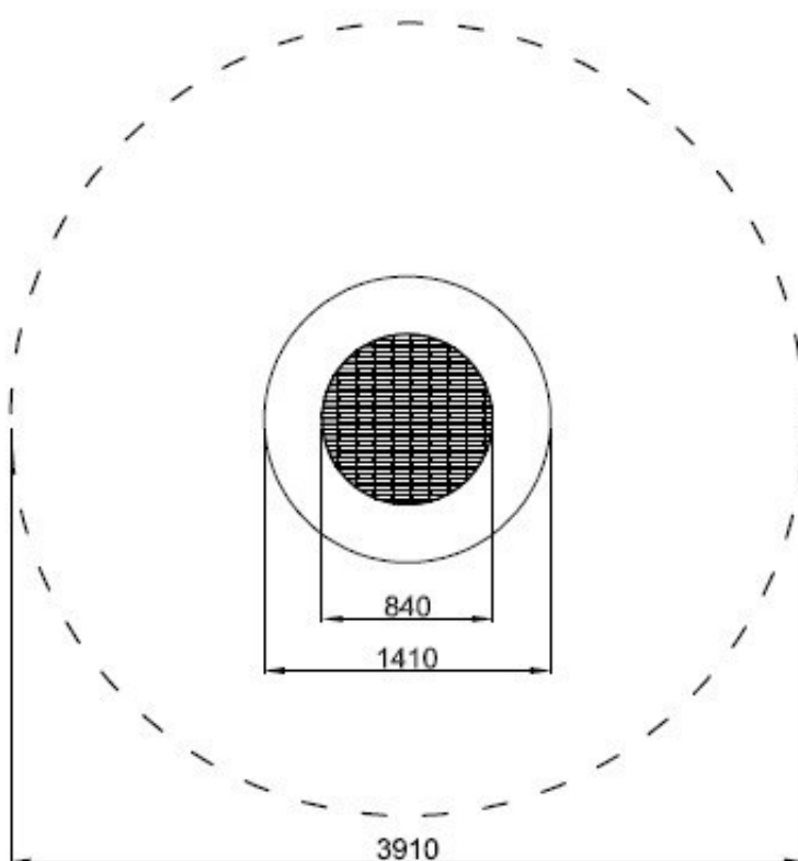
Att. 1 . Trampoline dimensions.
